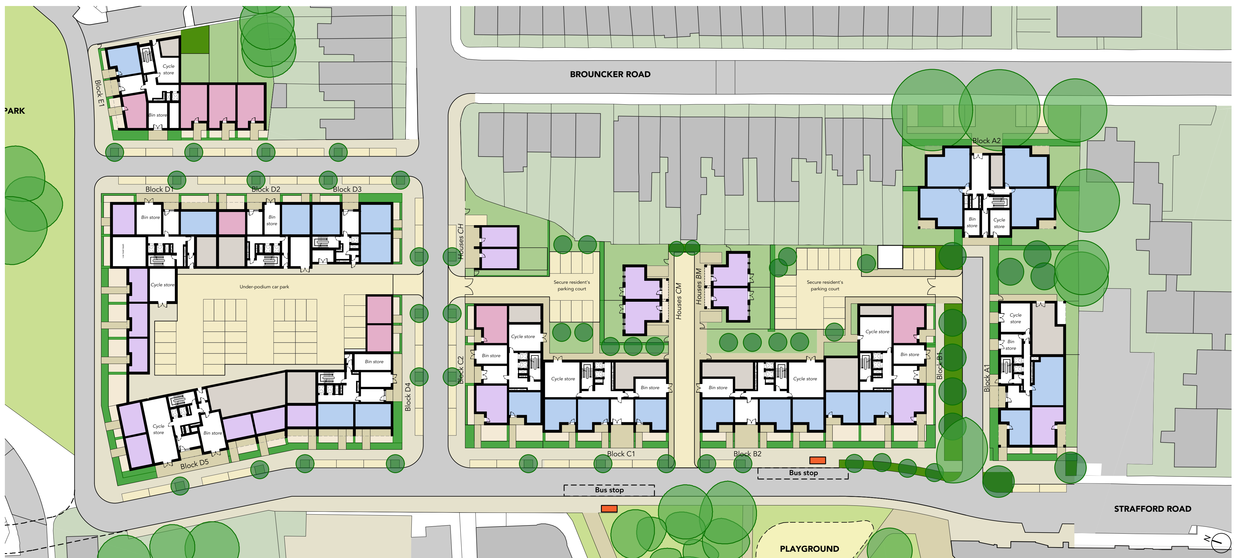
Above: Ground floor plan
